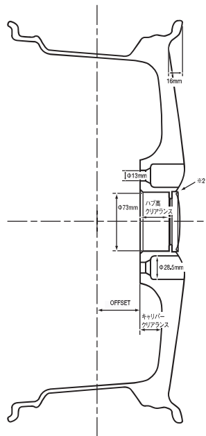
BUD F16 MONOBLOCK 18inch Center Section
