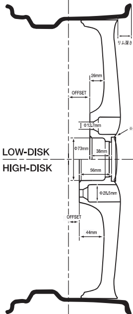
BUD F16 19inch Center Section
