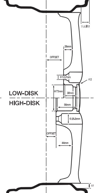
BUD F16 20inch Center Section
